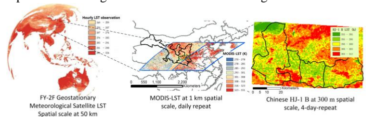
Figure 5. Remote sensing data play different roles in application according to their spatial and temporal difference. Data fusion suggests taking advantage of scale and repeat cycle.
