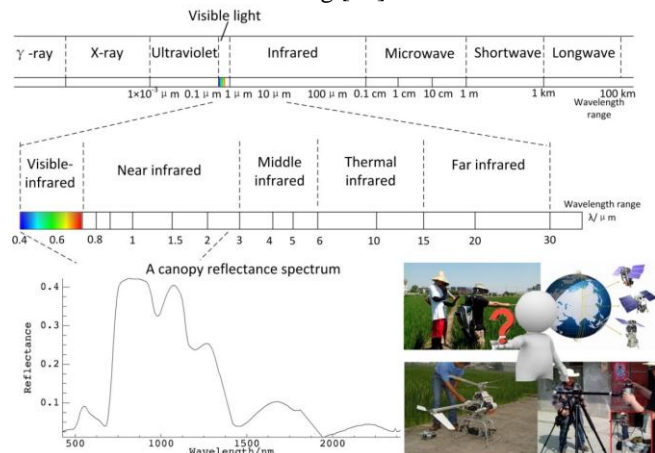
Figure 1. Illustration of electromagnetic spectral range, associated with sensors and platforms.
