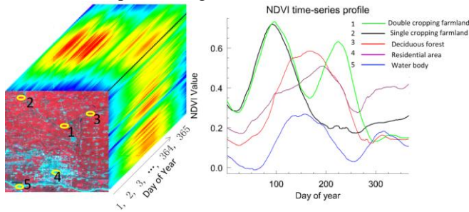
Figure 3. Time-series remote sensing data represents spatiotemporal characteristics of ground features.
