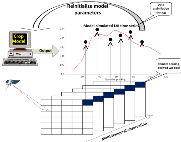
Figure 6. A simple schematic for assimilation of remote sensing data into crop models (the parameters optimization method).
