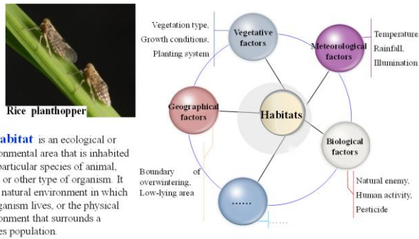
Figure 4. Identifying insect pests' habitat is helpful for early warning and prevention.
